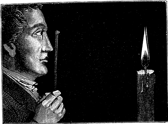
Fig. 18.—Aspect of a candle seen through a doubly-refractive crystal.
